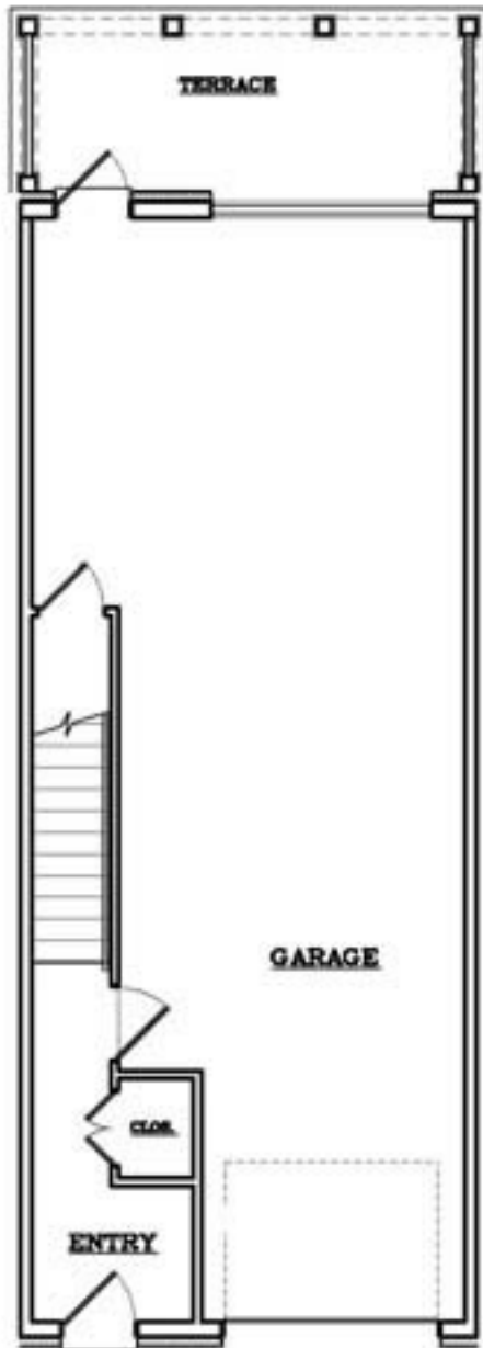
1 1st. LEVEL FLOOR PLAN AA.8 SCALE 1/4" = 1'-0" HAVEN
