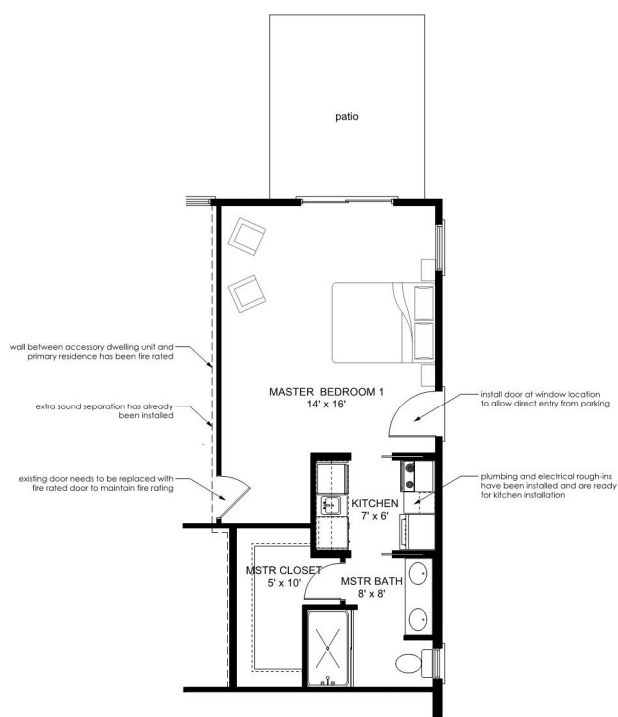
OPTIONAL CONVERSION GROUND FLOOR MASTER ACCESSORY DWELLING UNIT
