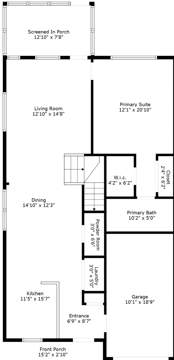
Floor 1
